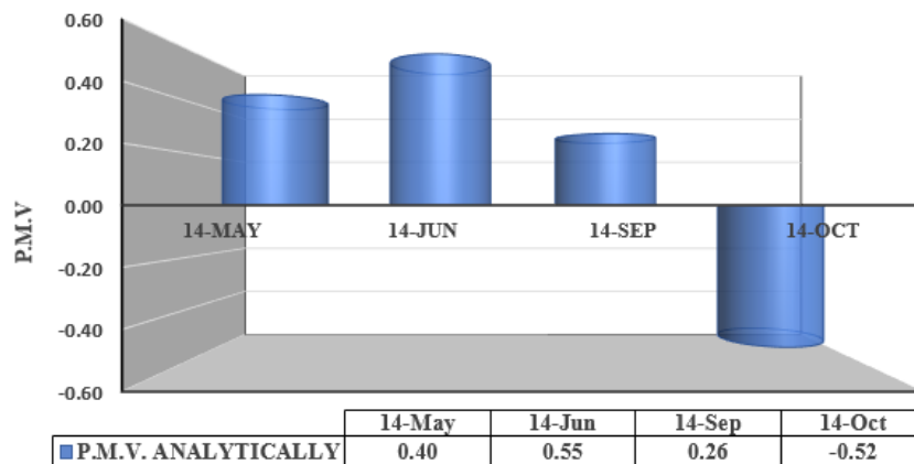
Chart 21. PMV values and comparison between the months on the same day
