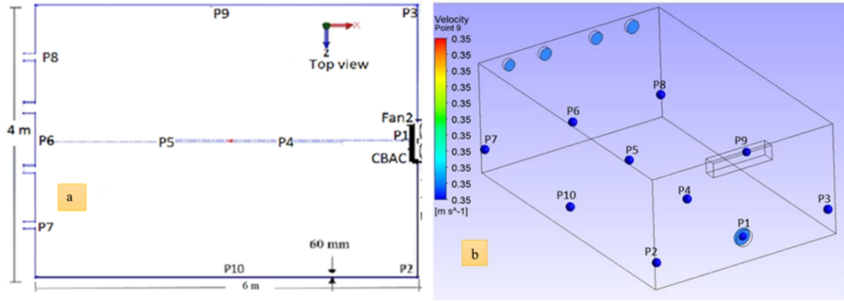
Figure 12. Positions of points at different locations inside E.C. a) researcher case and b) verification case 1
