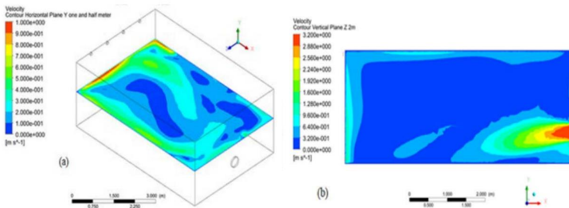
Figure 10. (a) Velocity contours horizontal plane 1.5 m (b) Velocity contours vertical plane 2 m for a researcher
