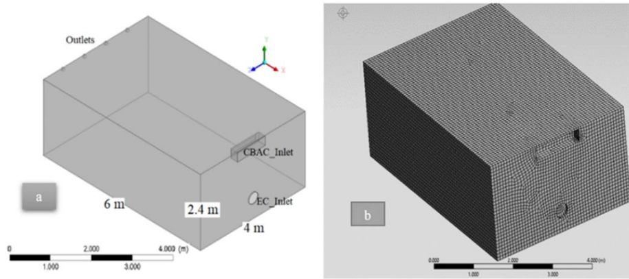
Figure 8. (a) Design room and (b) Mesh drawing a researcher
