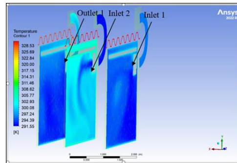
Figure 25. Three planes of temperature contour in two inlets and one outlet air
