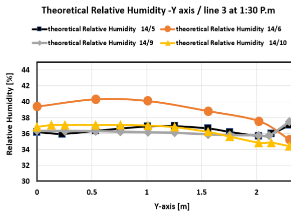
Chart 13. Relative humidity for four months at Z=2.5 m, X=0.85 m
