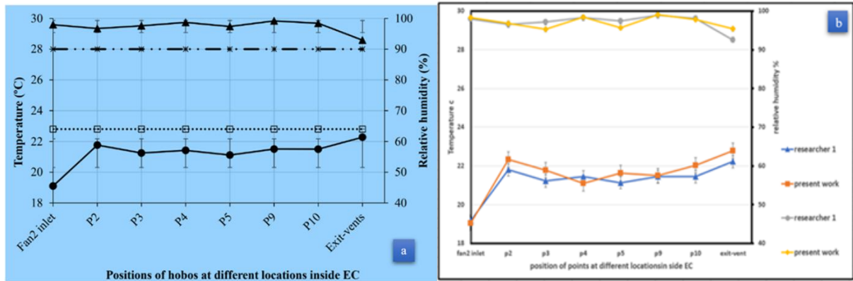
Chart 1. Comparison of measured and numerical values of temperature and relative humidity of the domain points a) researcher and b) verification case 1
