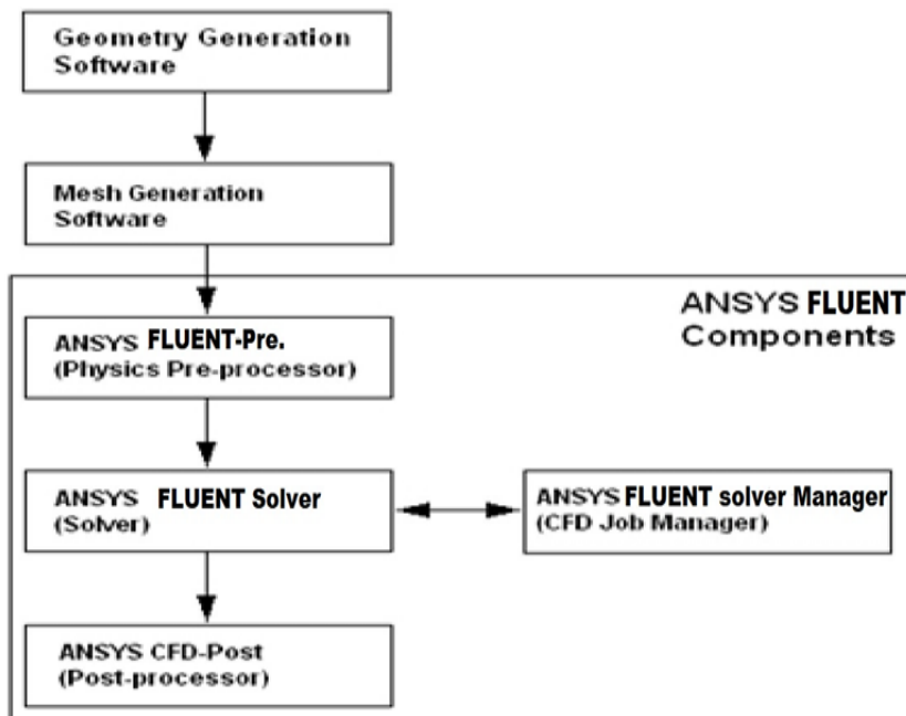
Figure 1. The structure of ANSYS Fluent; 1–Preprocessor, 2–Solver, 3–Post processor [21]
